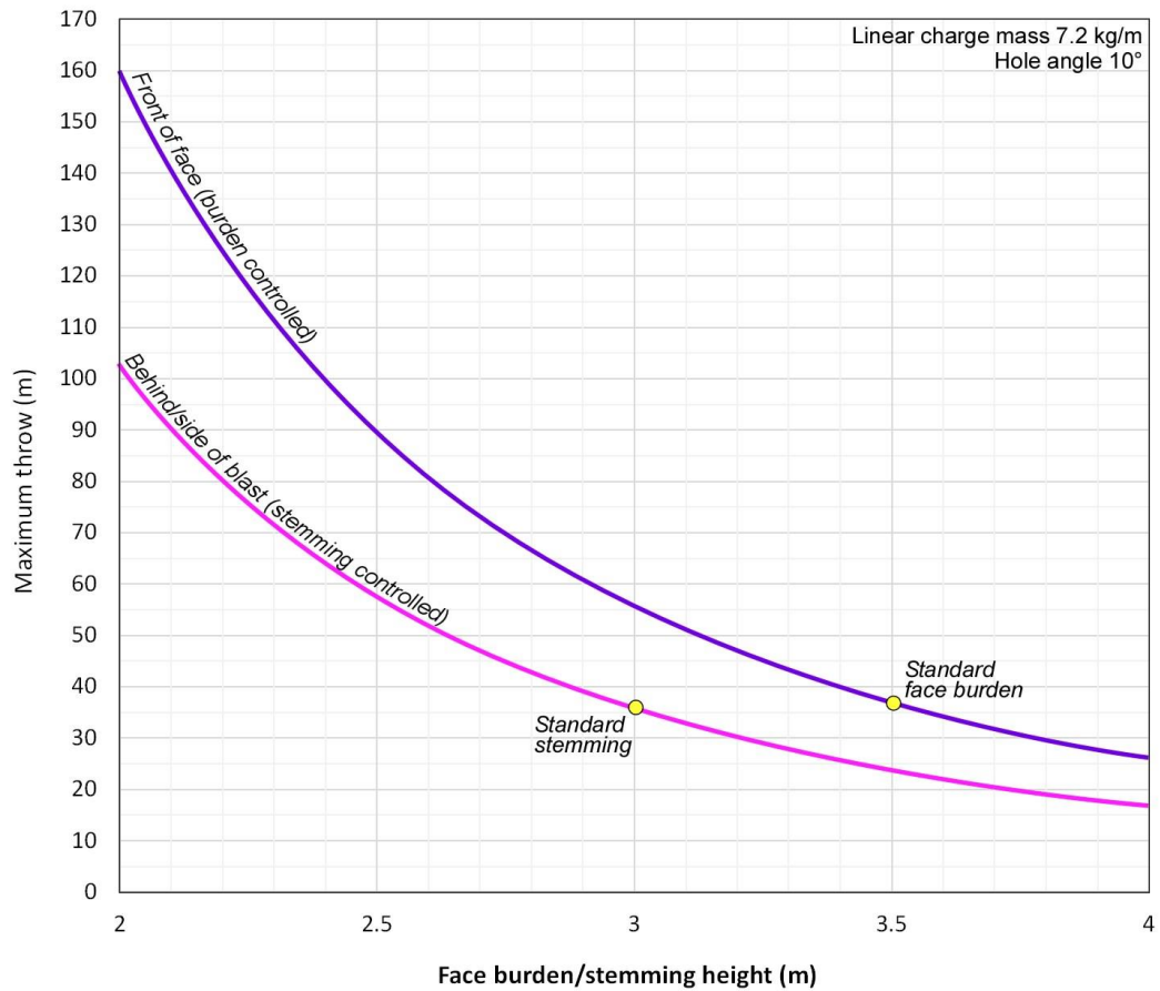
Figure 18 – Relationship between face burden/stemming and maximum throw
