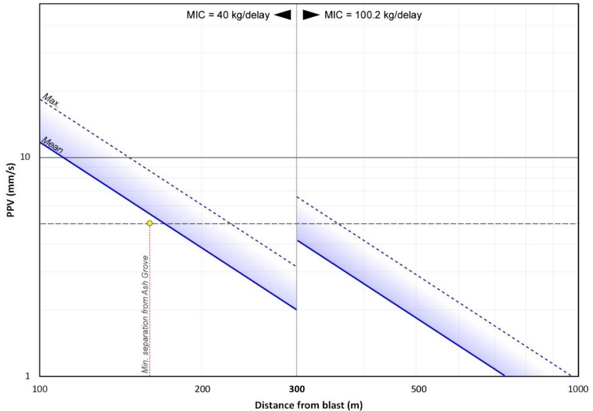
Figure 6 – Effect on PPV levels from reduced charge mass for blasts <300m from Ash Grove.
