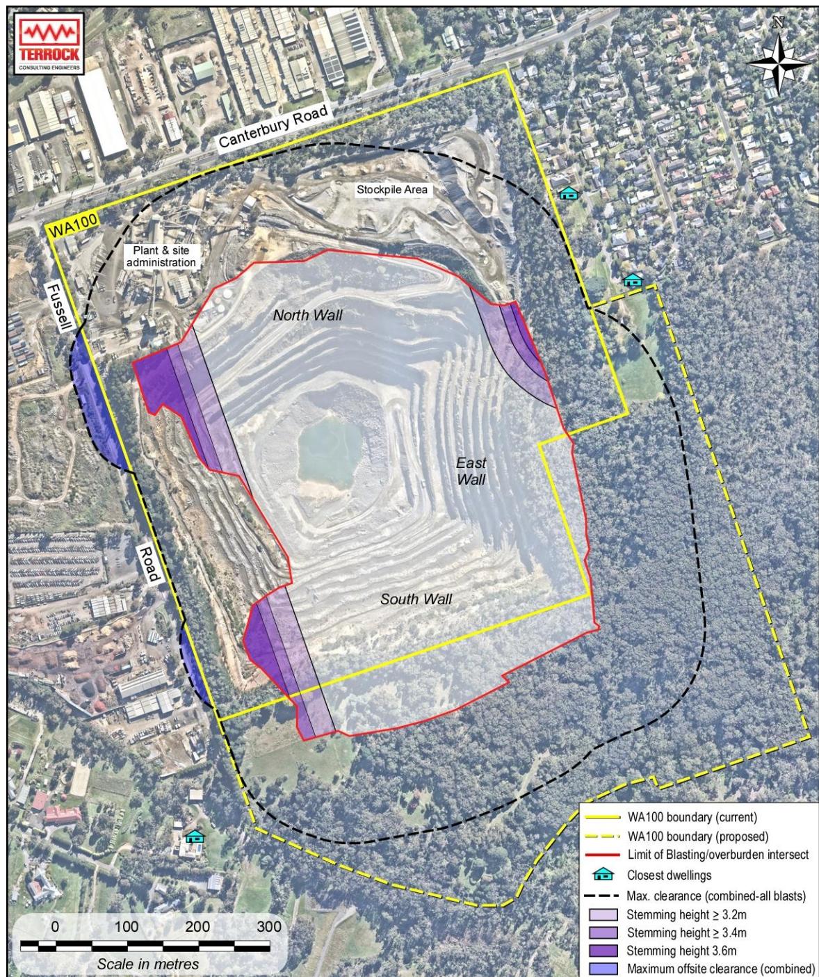
Figure 20 – Combined extent of blast clearance and stemming height requirements
