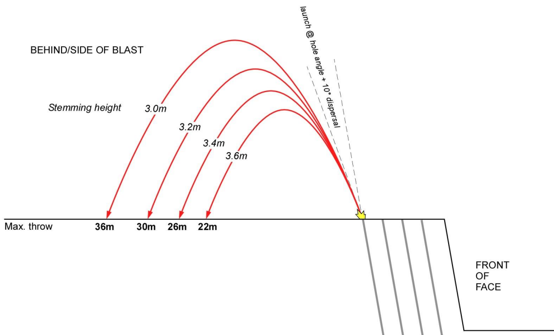
Figure 19 – Reduced maximum throw behind blasts from increased stemming heights
