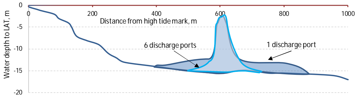
Figure 4. Maximum extent of cool water field cross-section (concept) One outlet and six-port discharge port options
