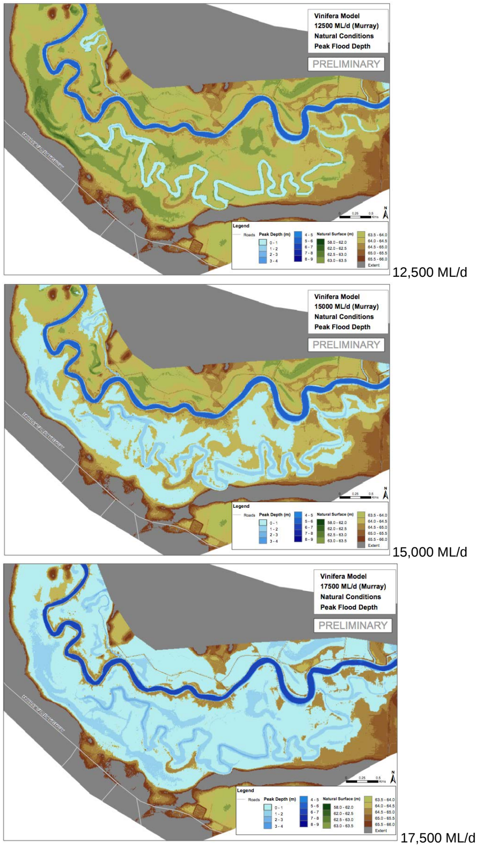
Figure 35. Vinifera floodplain inundation at flows of 12,500, 15,000 and 17,500 ML/d (Jacobs 2014).
