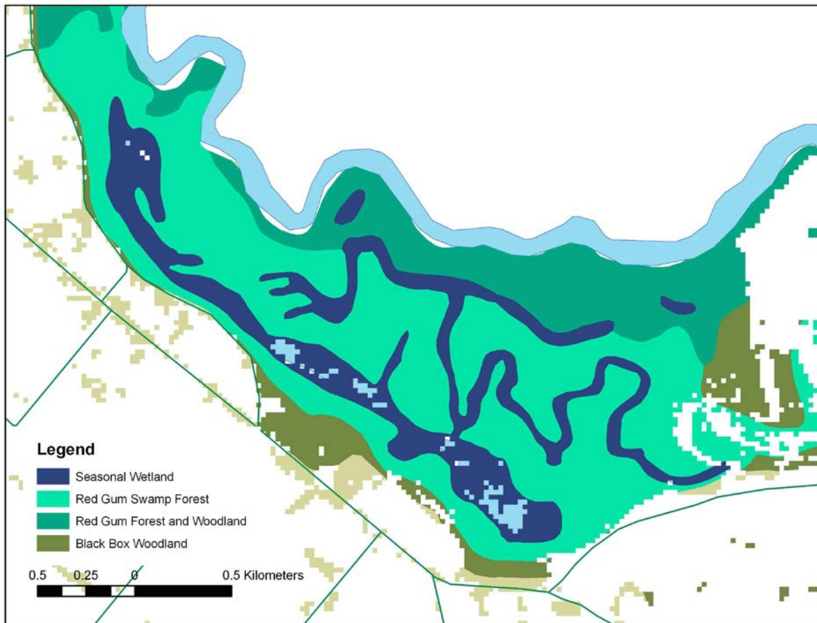
Figure 34. Vinifera Park Water Regime Classes
