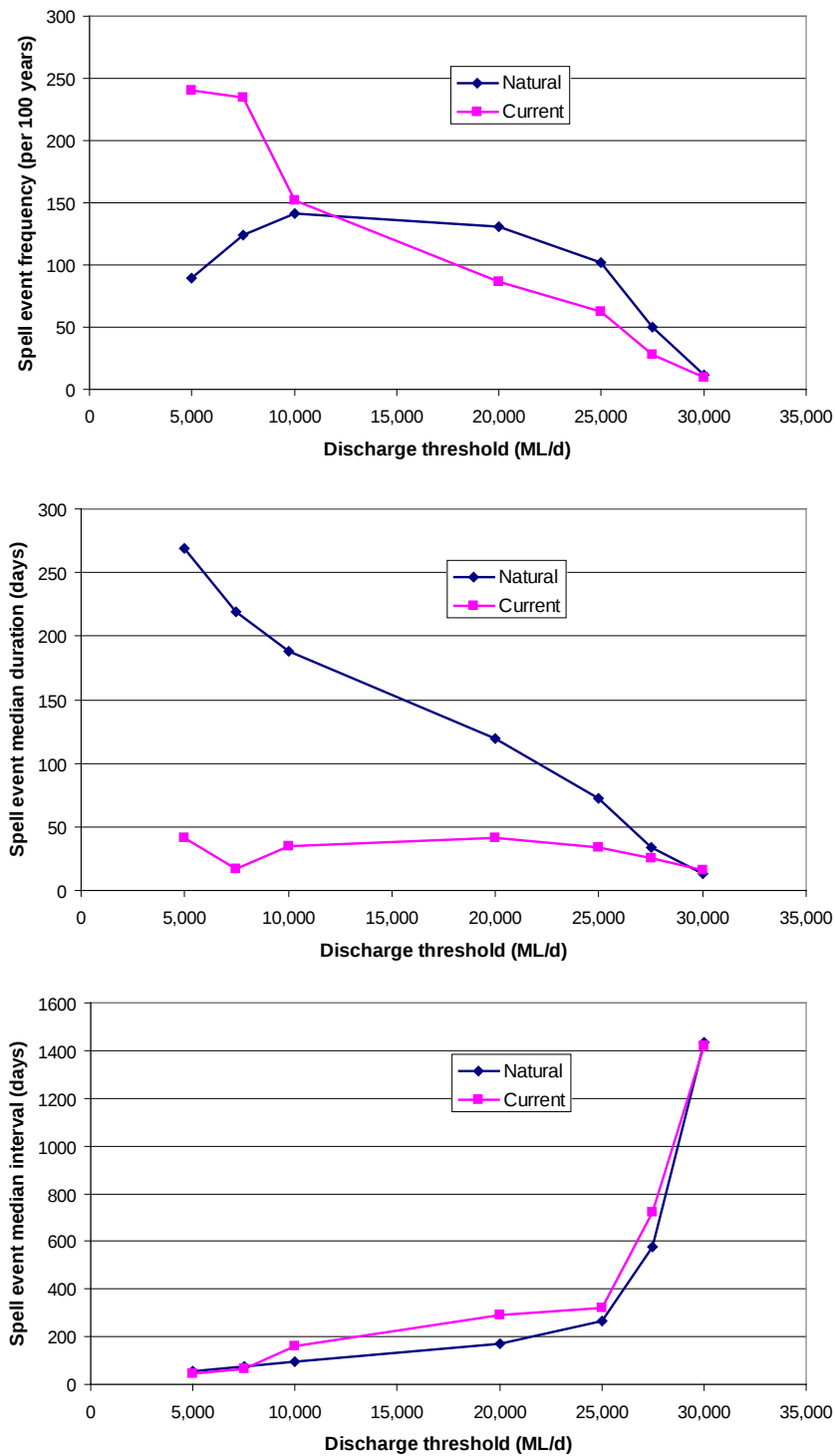
Figure 25. Spell event frequency, median duration and median interval for natural and current conditions (Swan Hill gauge). Derived from MDBC MSM-Bigmod 109 year data (Ecological Associates 2006)
