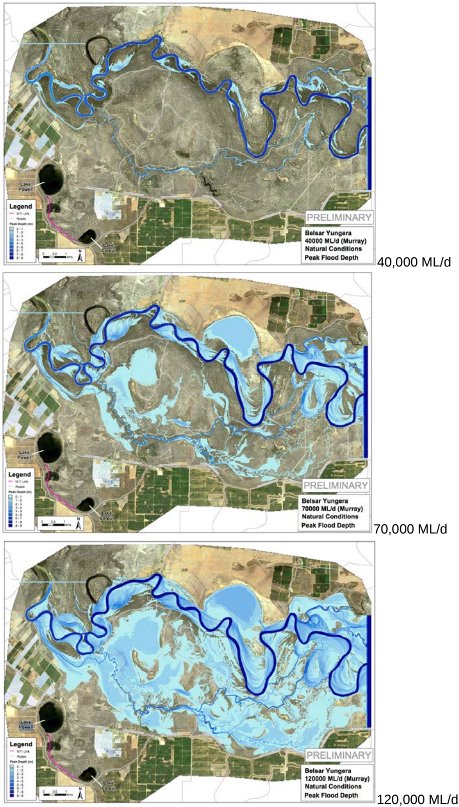
Figure 17. Belsar Yungera floodplain inundation at flows of 40,000, 70,000 and 120,000 ML/d (data supplied by Water Technology).
