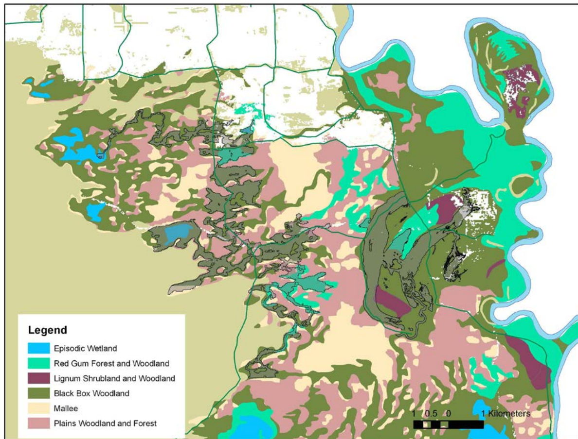
Figure 14. Water regime classes inundated by proposed works in Hattah North
