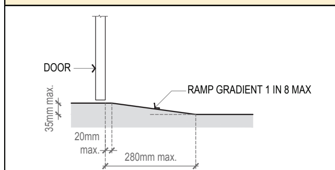
Figure 3.3: Threshold ramp section at the apartment entrance
