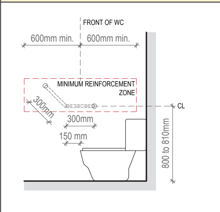
Figure 3.6: Toilet wall reinforcement elevation for future grab rails
