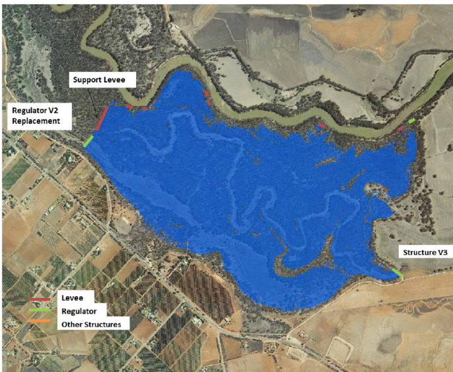
Figure 2 Vinifera extent of flooding – option 2 (figure sourced from GHD, 2014 and reproduced from Alluvium, 2013)
