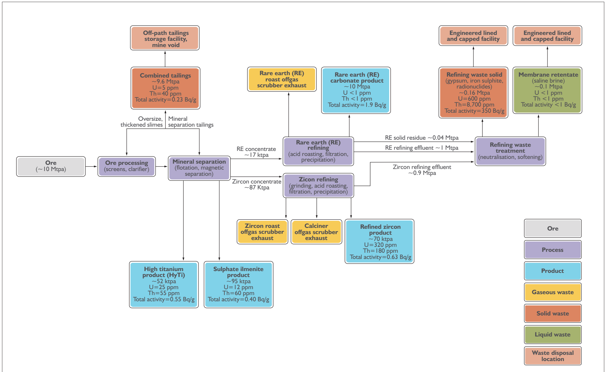
Processing and refining flowchart – option A – engineered cells
