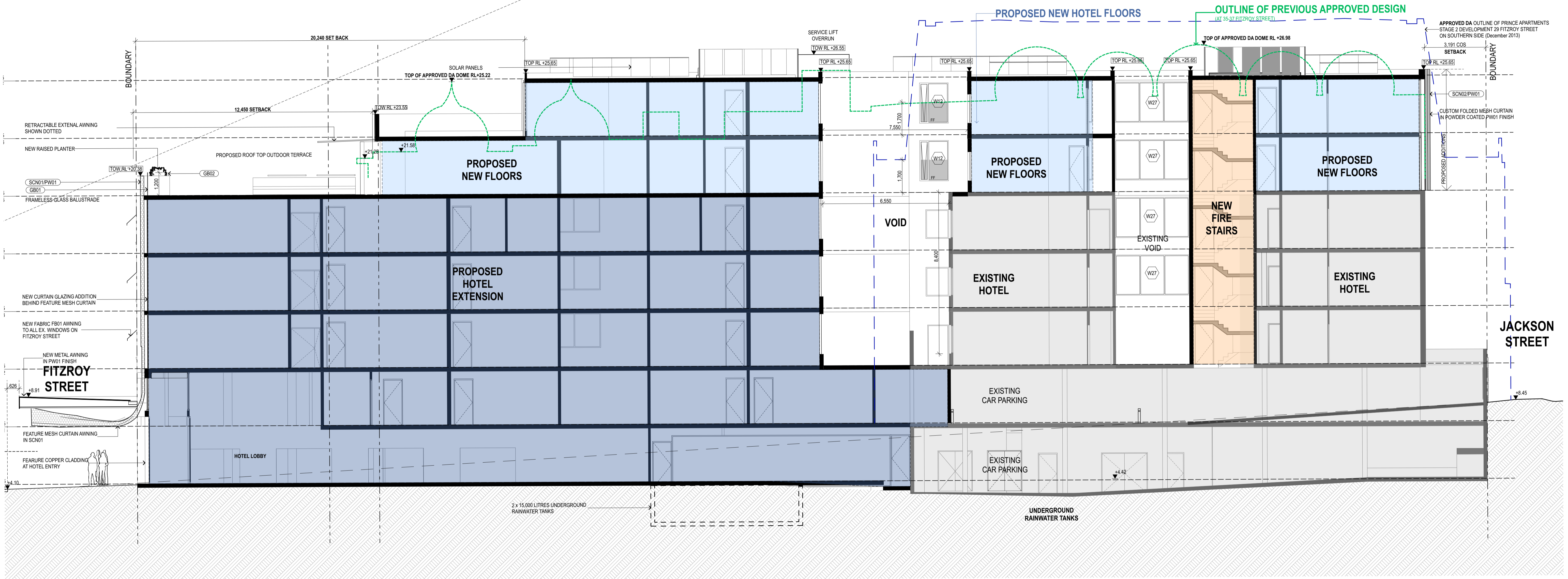
1 LONG SECTION 1:100
