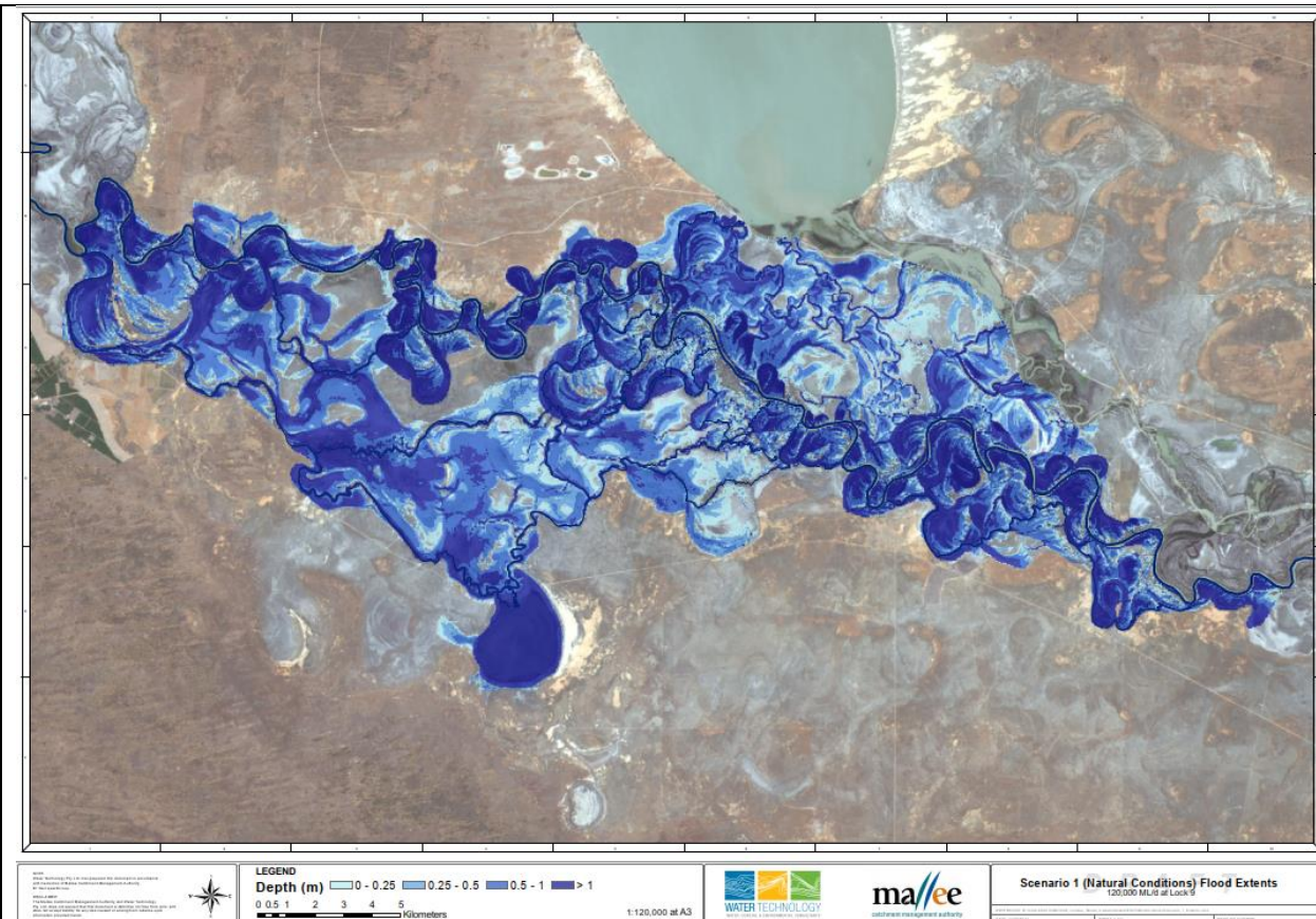
120,000 ML/day Flood Extents (Natural Conditions)
