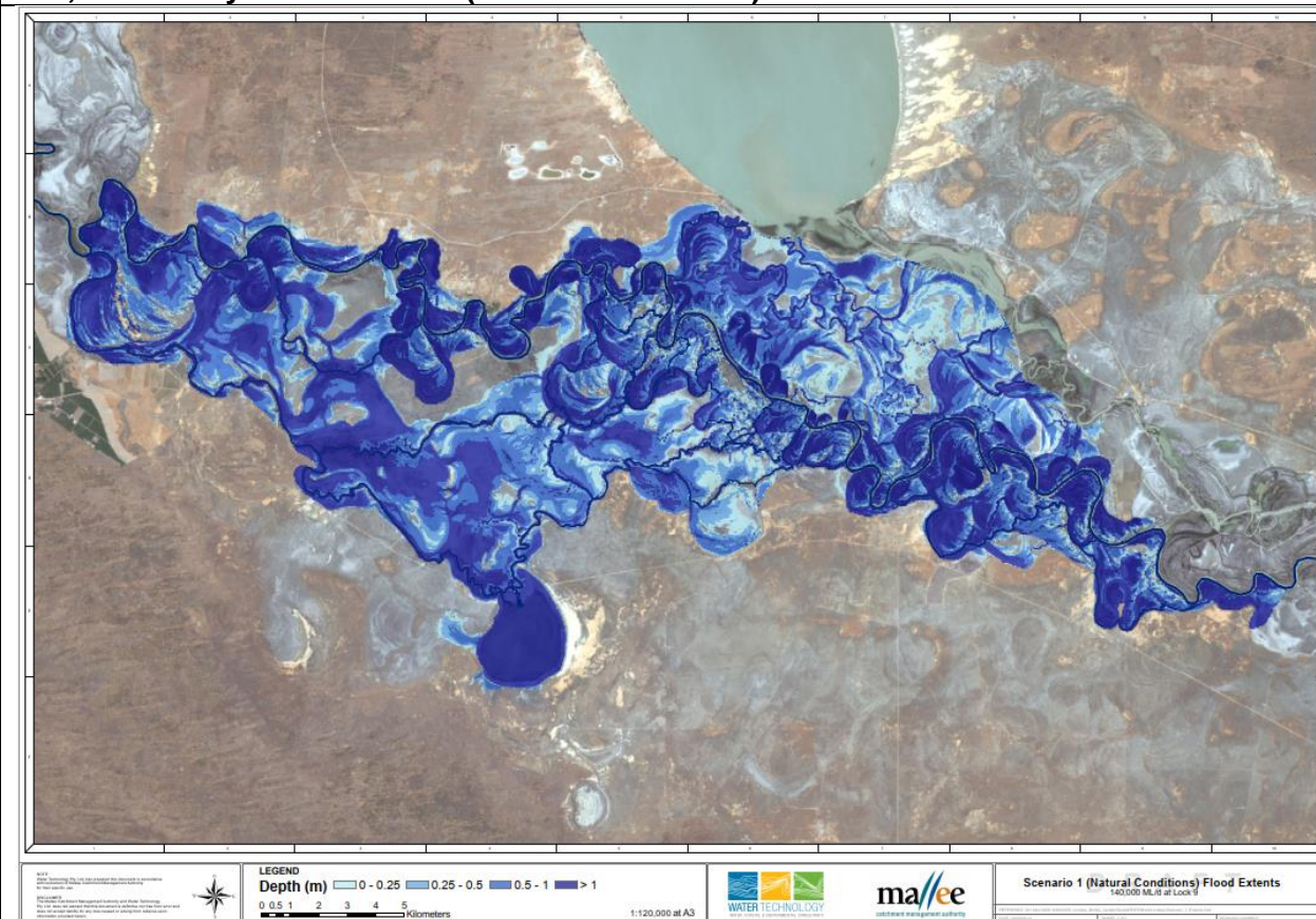
140,000 ML/day Flood Extents (Natural Conditions)
