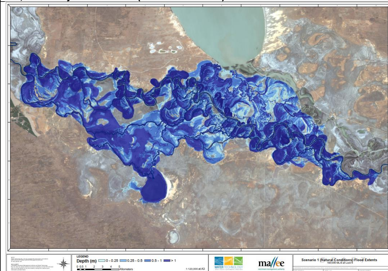
160,000 ML/day Flood Extents (Natural Conditions)
