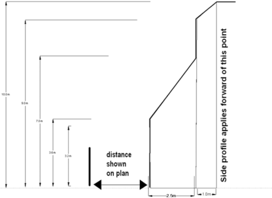
Rear profile RP-X - setback of first wall from rear boundary is shown on a plan
